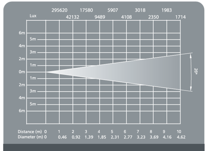
Beam angle 26°
