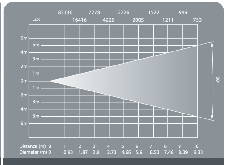
Beam angle 50°
